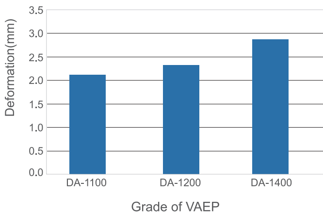
Tile adhesive transverse deformation test (EN-12002) 磁磚接著砂漿柔軟性測試 (EN-12002)
